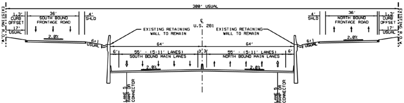
PROPOSED U.S. 281
