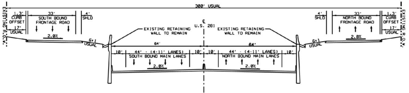
EXISTING U.S. 281
